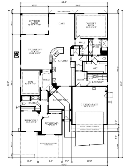
Floor Plan
