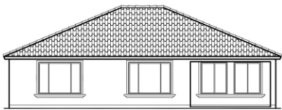
Rear Elevation
