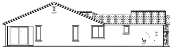
Left Elevation
