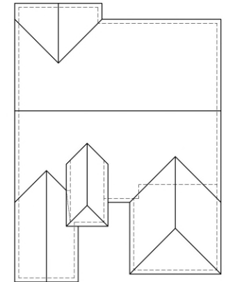
Roof Plan
