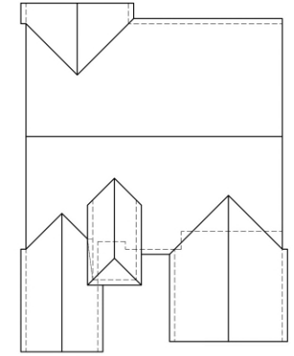
Roof Plan
