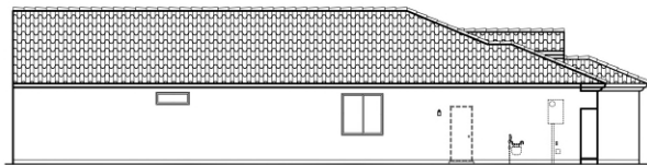
Left Elevation
