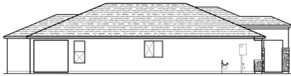
Left Elevation
