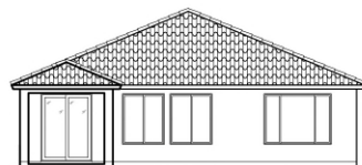
Rear Elevation
